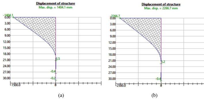
Gambar 7. Hasil displacement: (a) muka air banjir, (b) muka air normal
